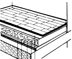
⑬ Finished parquet elements on floor screed
